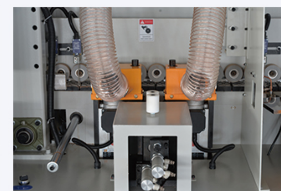
Pre-milling unit with diamond cutters
