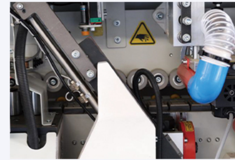
End cutting unit with high speed motor
